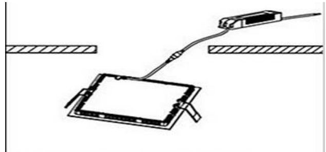
Take DC conector to the power supply
