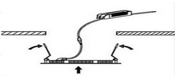
Plug the jump ring and put the lights into the ceiling
